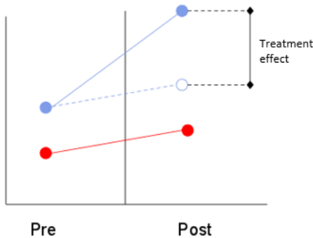
Figure 1. Estimating Treatment Effects Using DiD Approach
